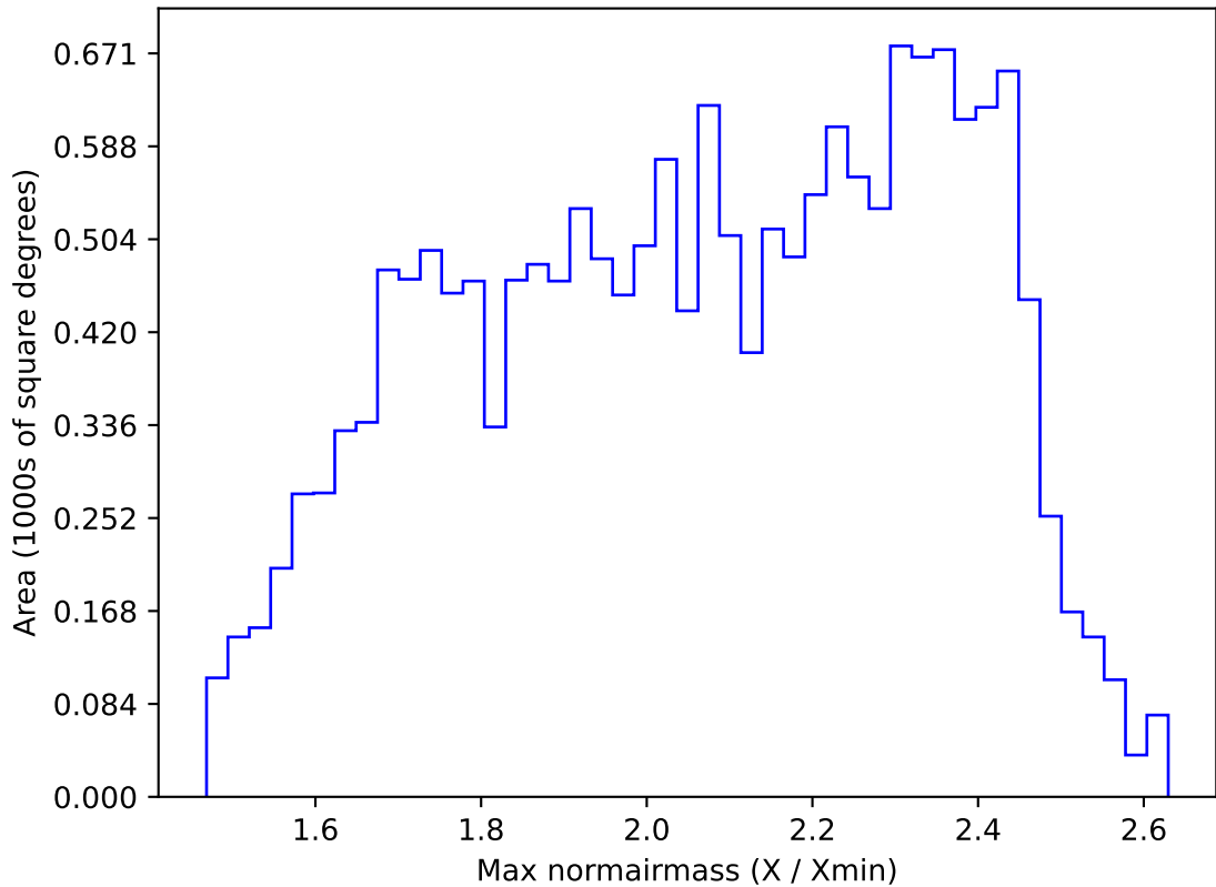
ddf_loaded_half_fl1_v3.4_10yrs WFD r band: Max normairmass
