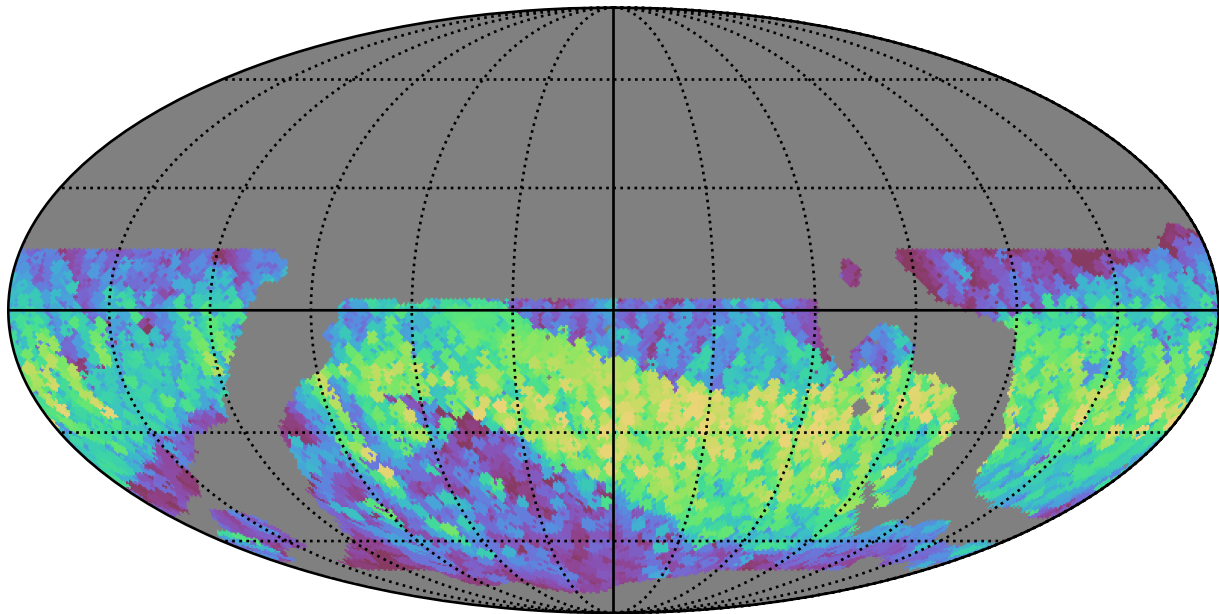
ddf_loaded_half_fl1_v3.4_10yrs WFD i band: Max normairmass
