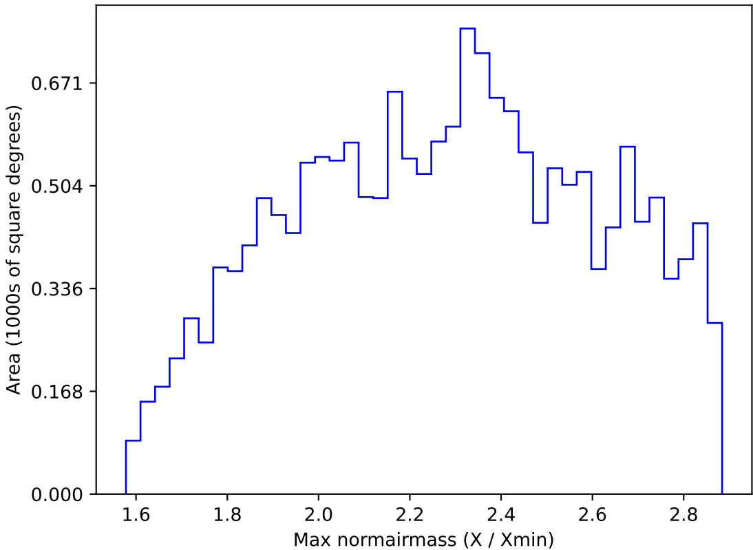
ddf_loaded_half_fl1_v3.4_10yrs WFD i band: Max normairmass
