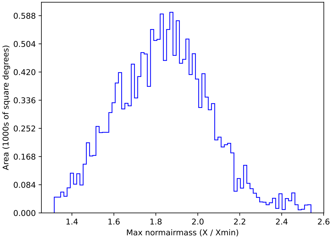
ddf_loaded_half_fl1_v3.4_10yrs WFD g band: Max normairmass
