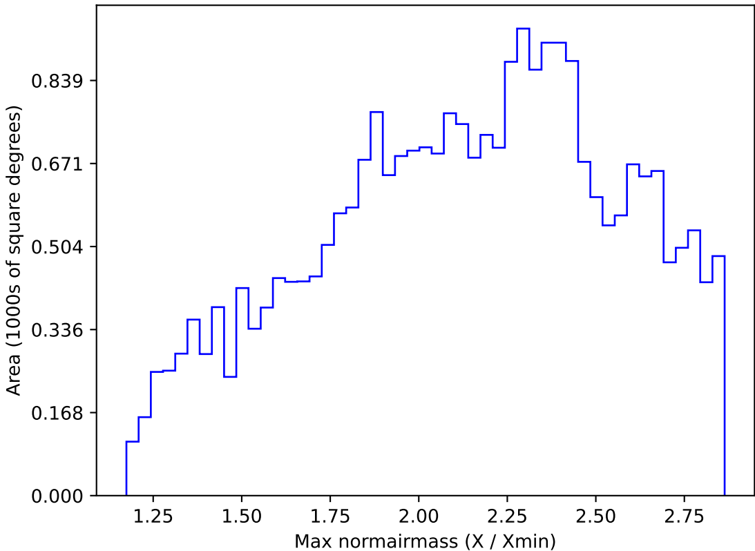
ddf_loaded_half_fl1_v3.4_10yrs All sky z band: Max normairmass
