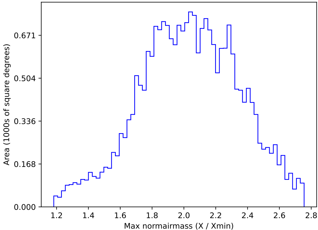
ddf_loaded_half_fl1_v3.4_10yrs All sky y band: Max normairmass
