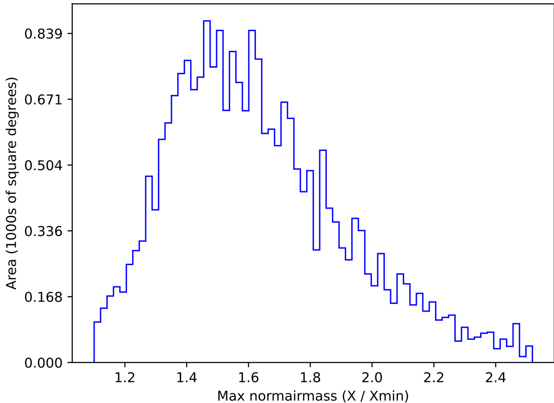
ddf_loaded_half_fl1_v3.4_10yrs All sky u band: Max normairmass
