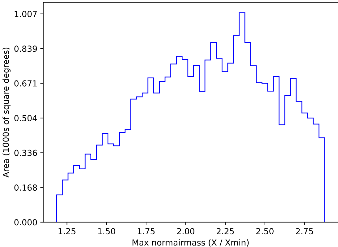
ddf_loaded_half_fl1_v3.4_10yrs All sky i band: Max normairmass
