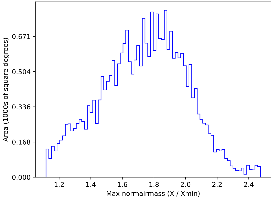
ddf_loaded_half_fl1_v3.4_10yrs All sky g band: Max normairmass
