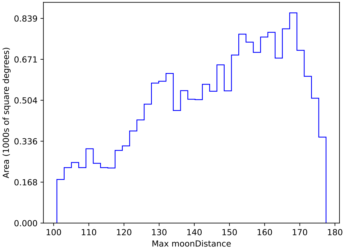
ddf_loaded_half_fl1_v3.4_10yrs WFD y band: Max moonDistance
