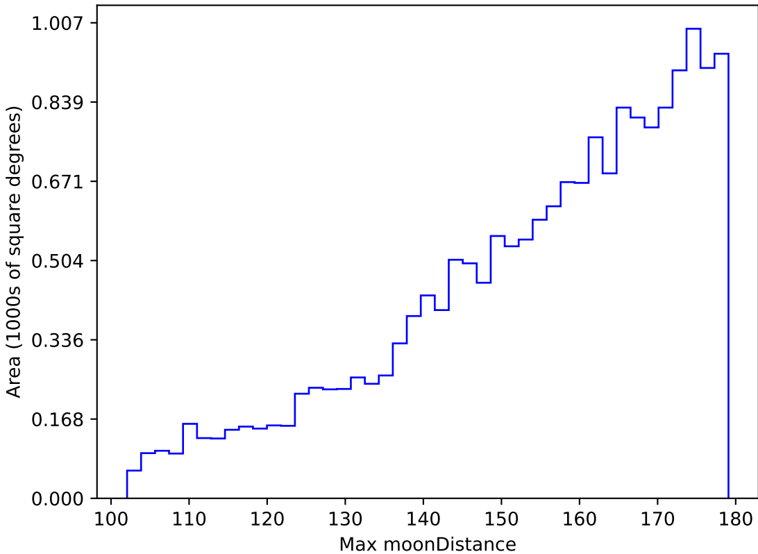
ddf_loaded_half_fl1_v3.4_10yrs WFD u band: Max moonDistance
