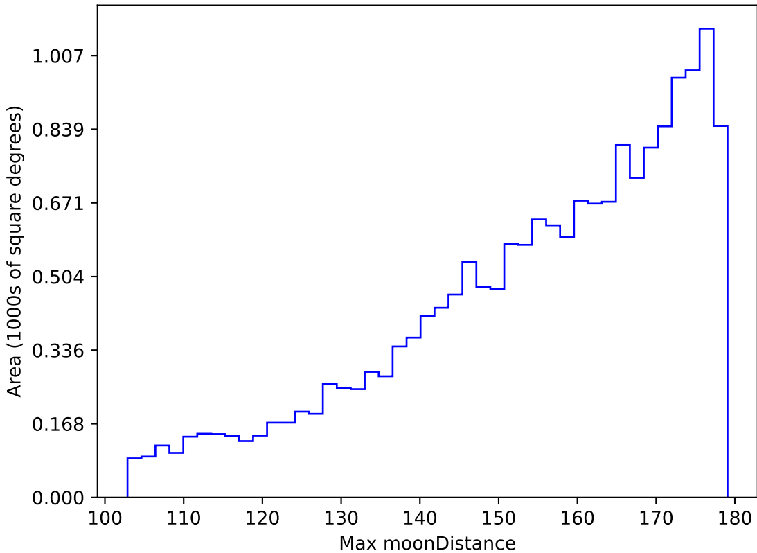
ddf_loaded_half_fl1_v3.4_10yrs WFD g band: Max moonDistance
