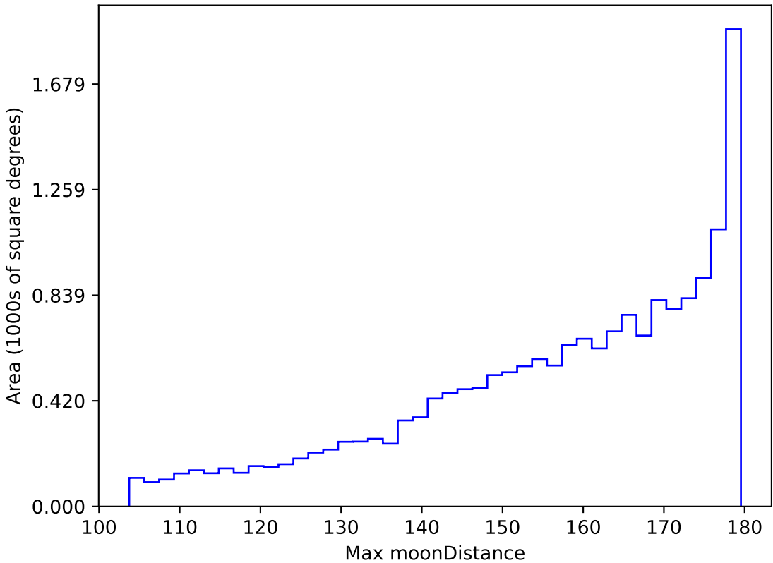
ddf_loaded_half_fl1_v3.4_10yrs WFD all bands: Max moonDistance
