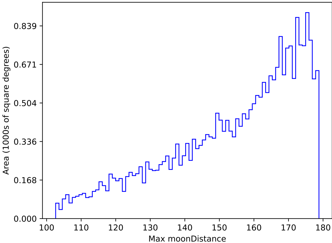
ddf_loaded_half_fl1_v3.4_10yrs All sky z band: Max moonDistance
