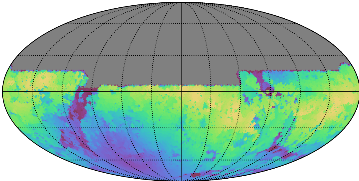
ddf_loaded_half_fl1_v3.4_10yrs All sky y band: Max moonDistance
