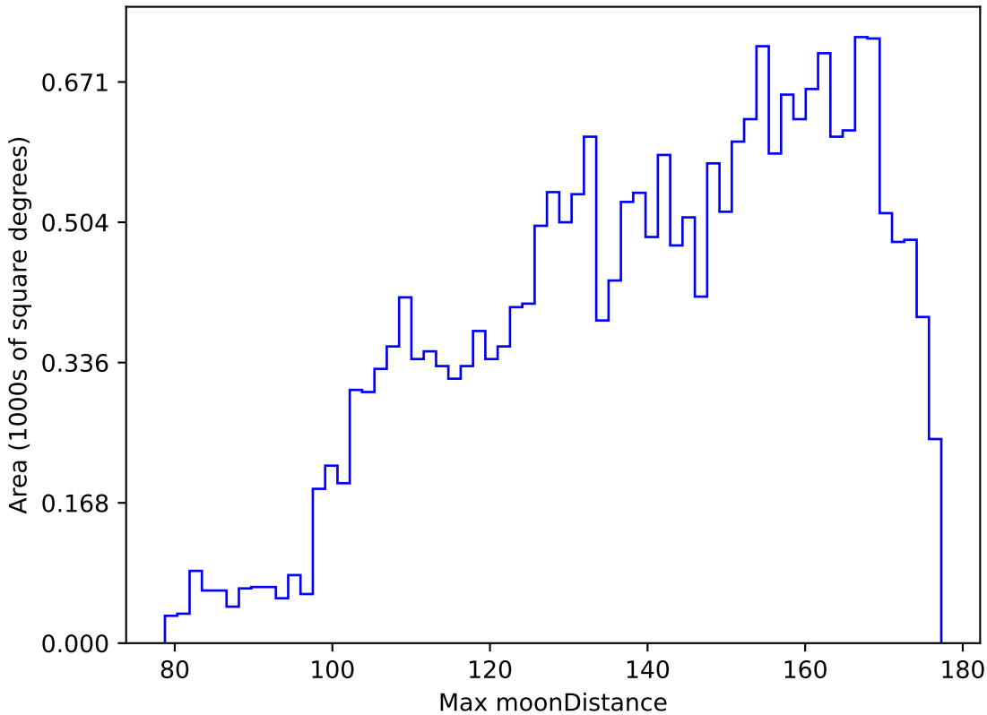
ddf_loaded_half_fl1_v3.4_10yrs All sky y band: Max moonDistance
