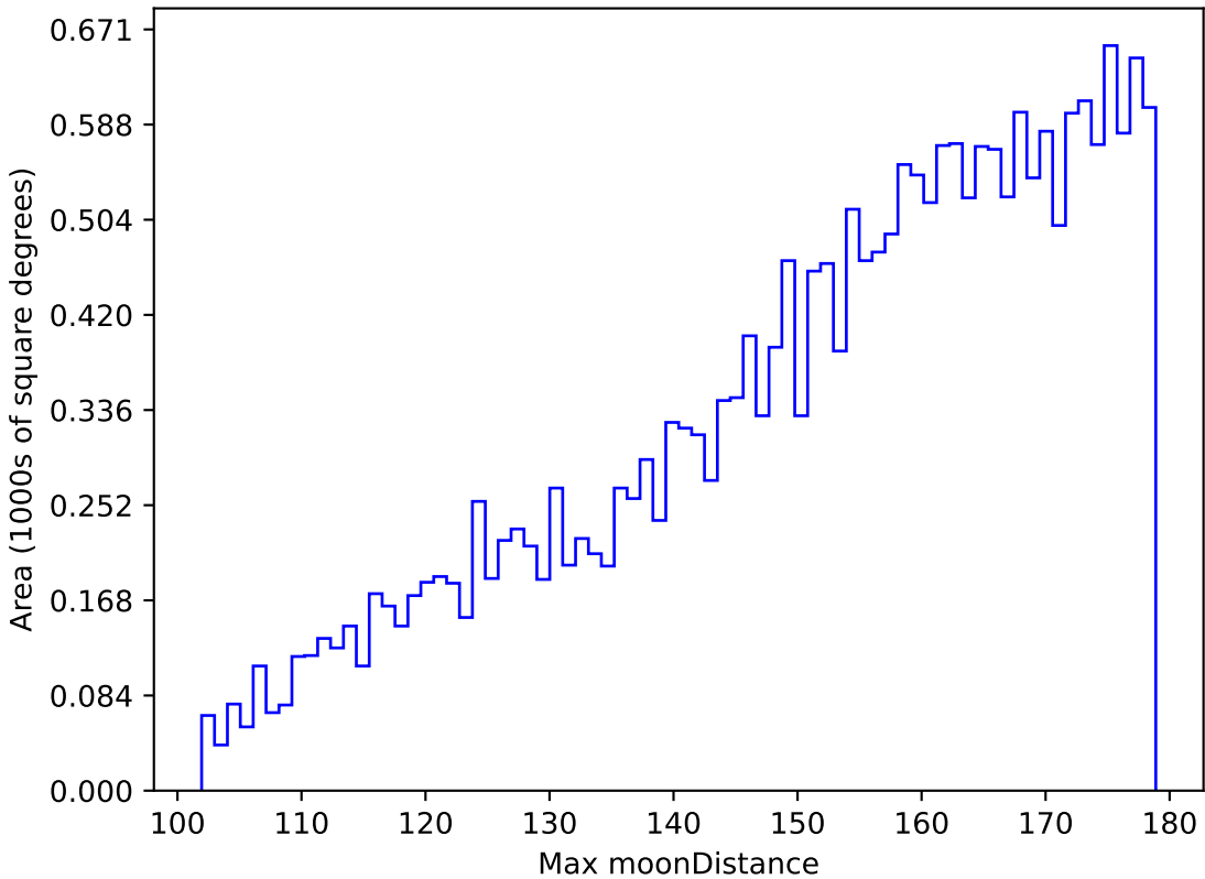
ddf_loaded_half_fl1_v3.4_10yrs All sky u band: Max moonDistance
