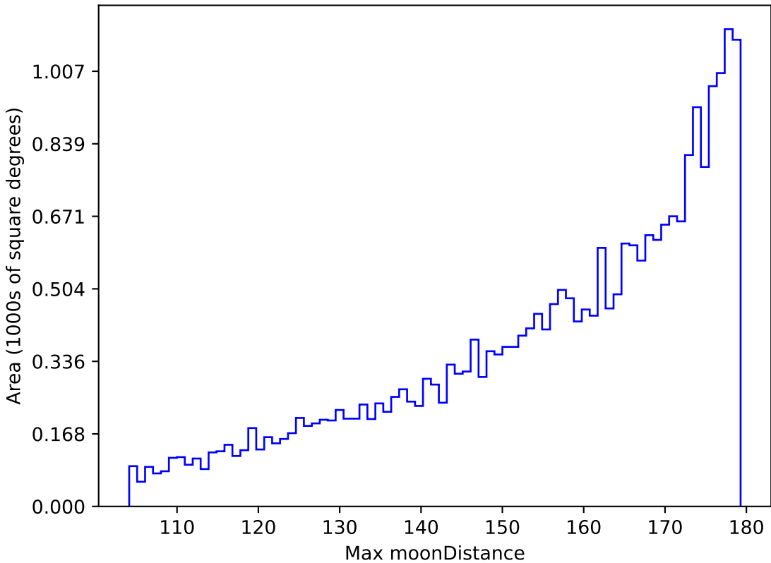
ddf_loaded_half_fl1_v3.4_10yrs All sky r band: Max moonDistance
