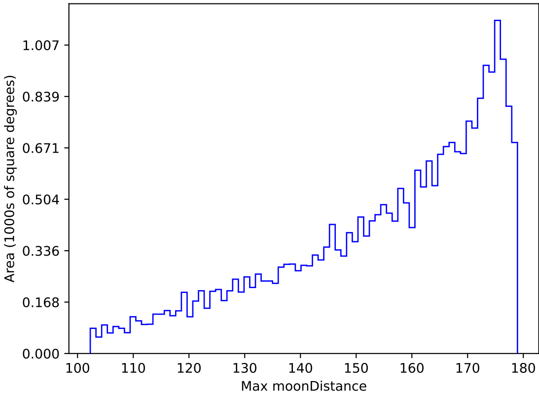
ddf_loaded_half_fl1_v3.4_10yrs All sky g band: Max moonDistance
