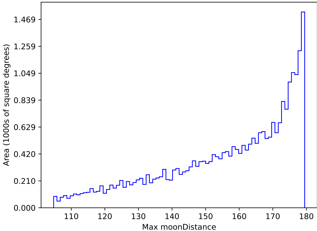
ddf_loaded_half_fl1_v3.4_10yrs All sky all bands: Max moonDistance
