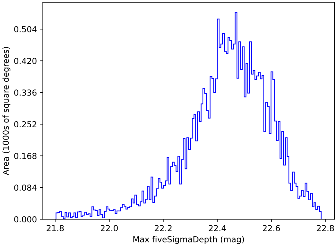
ddf_loaded_half_fl1_v3.4_10yrs Yr 1 y band: Max fiveSigmaDepth
