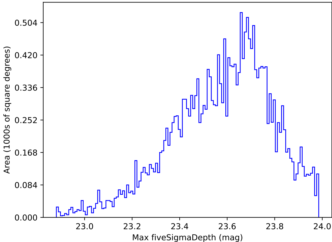
ddf_loaded_half_fl1_v3.4_10yrs Yr 1 u band: Max fiveSigmaDepth
