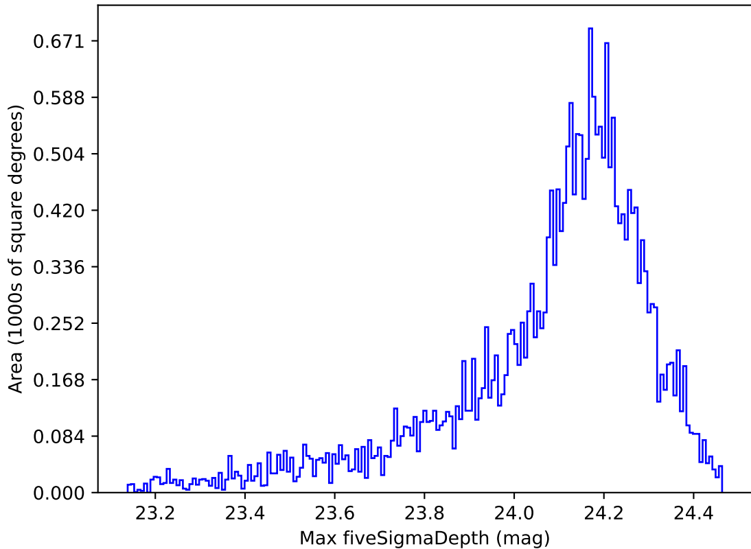
ddf_loaded_half_fl1_v3.4_10yrs Yr 1 i band: Max fiveSigmaDepth
