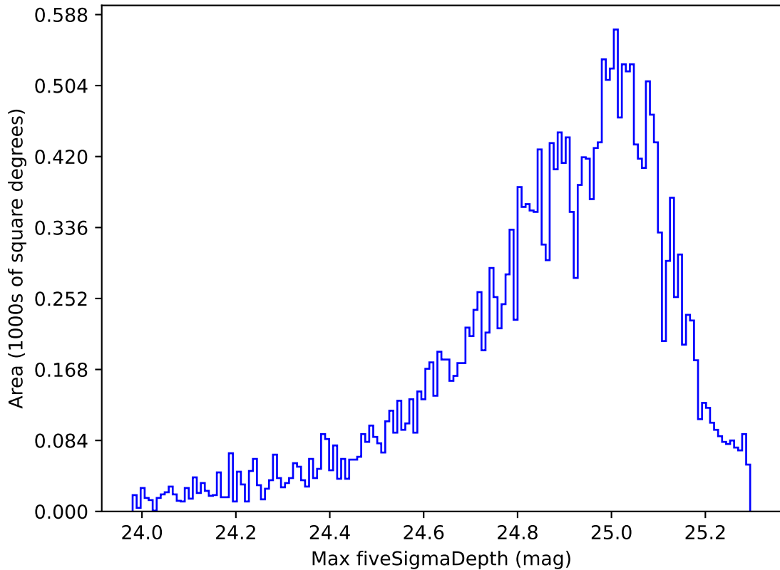
ddf_loaded_half_fl1_v3.4_10yrs Yr 1 g band: Max fiveSigmaDepth
