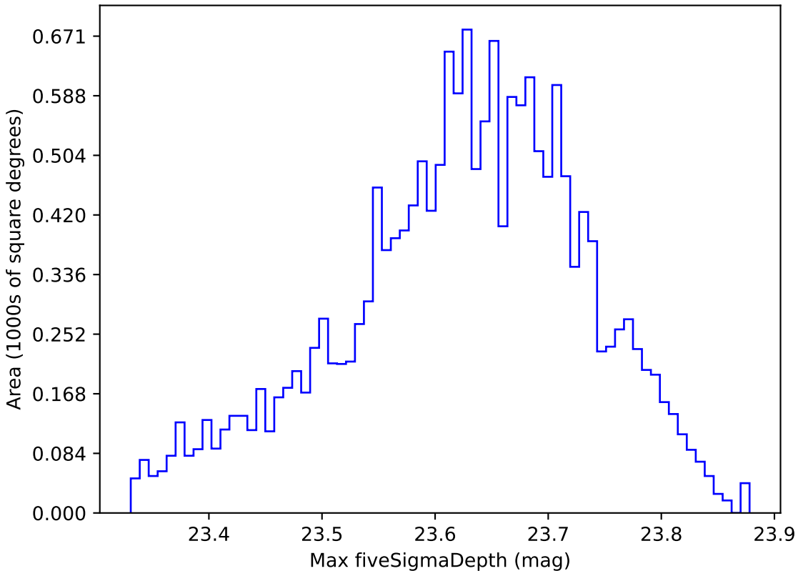
ddf_loaded_half_fl1_v3.4_10yrs WFD z band: Max fiveSigmaDepth
