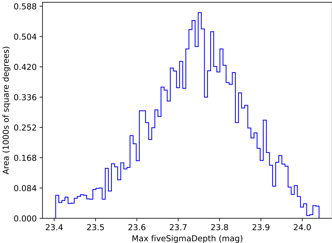
ddf_loaded_half_fl1_v3.4_10yrs WFD u band: Max fiveSigmaDepth
