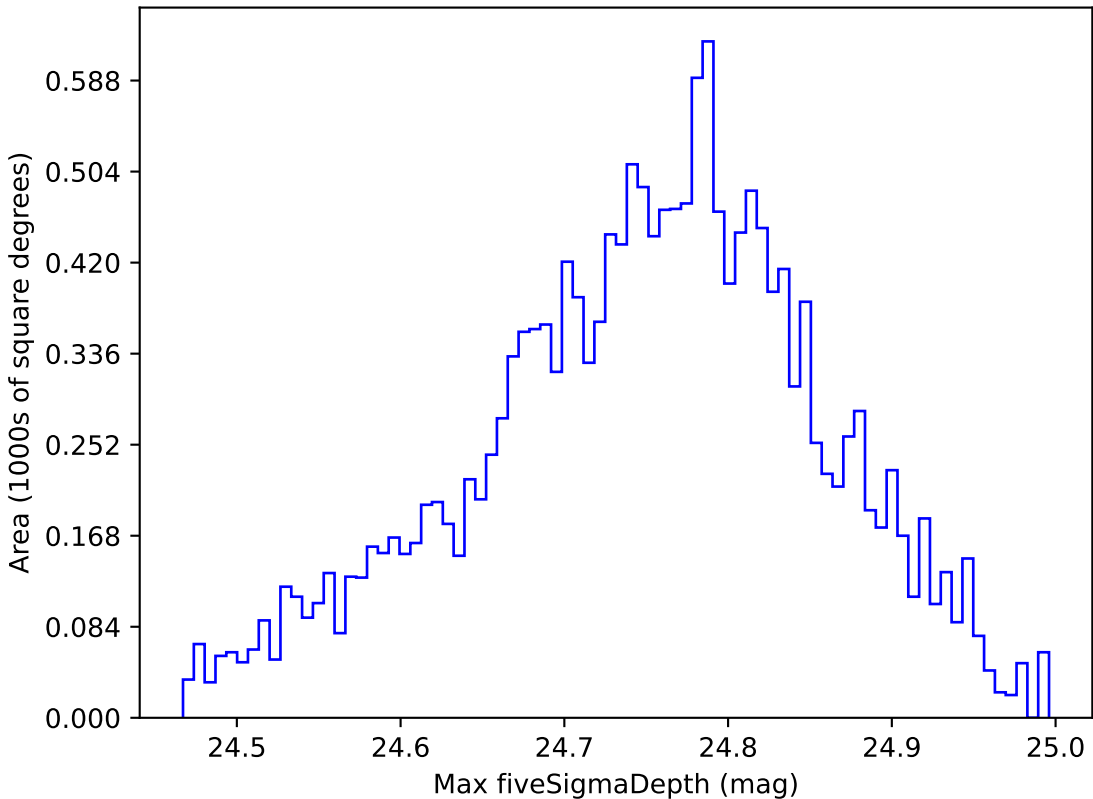
ddf_loaded_half_fl1_v3.4_10yrs WFD r band: Max fiveSigmaDepth
