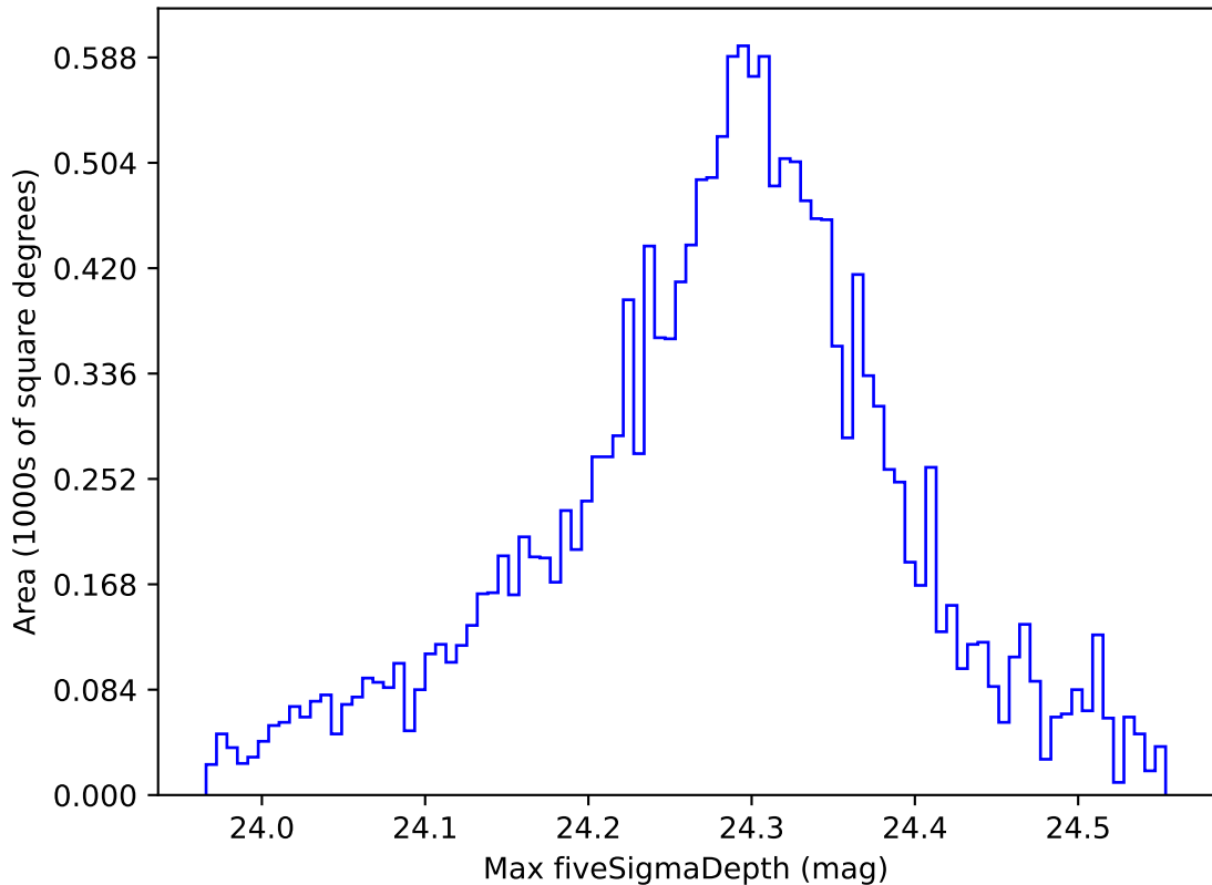
ddf_loaded_half_fl1_v3.4_10yrs WFD i band: Max fiveSigmaDepth
