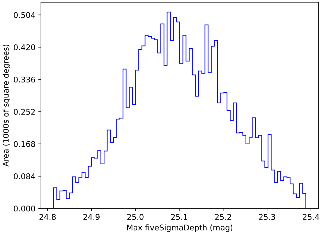
ddf_loaded_half_fl1_v3.4_10yrs WFD g band: Max fiveSigmaDepth
