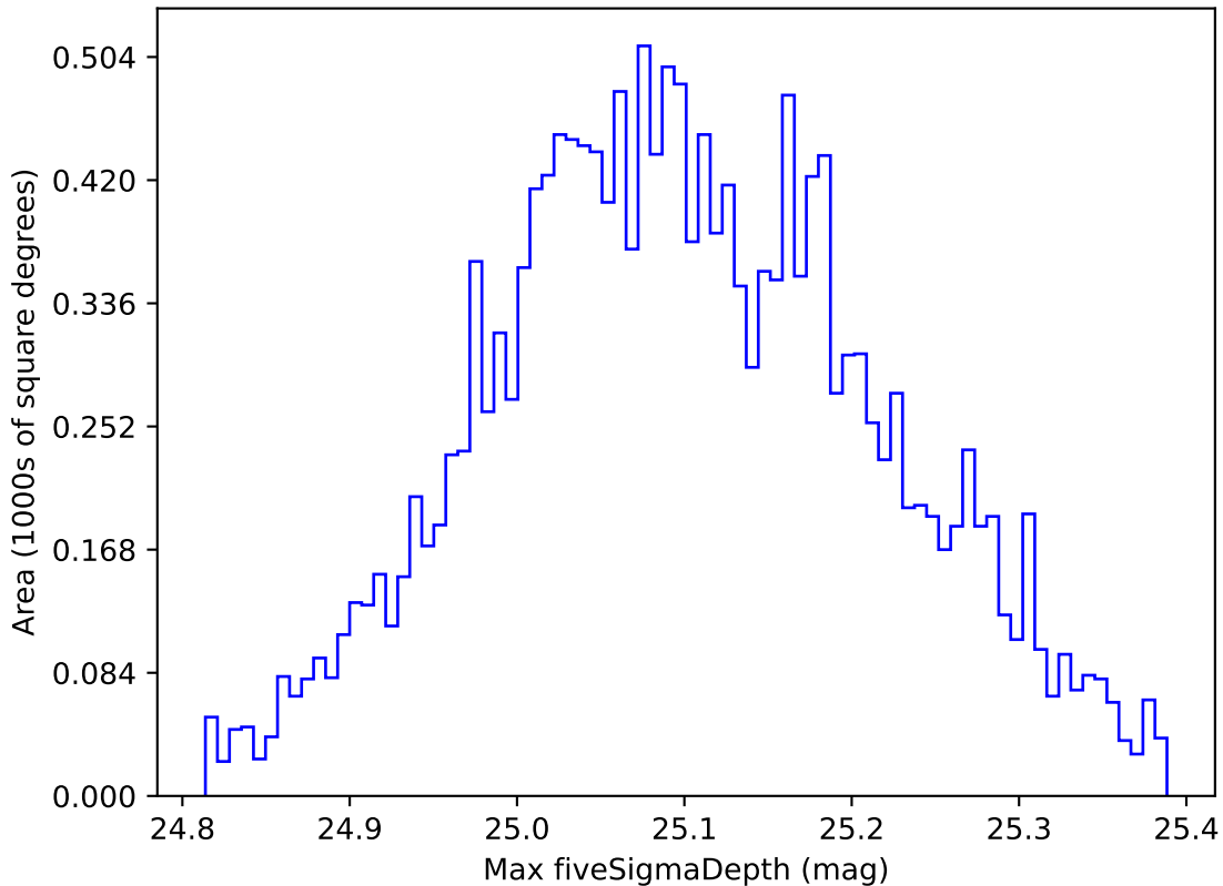
ddf_loaded_half_fl1_v3.4_10yrs WFD all bands: Max fiveSigmaDepth
