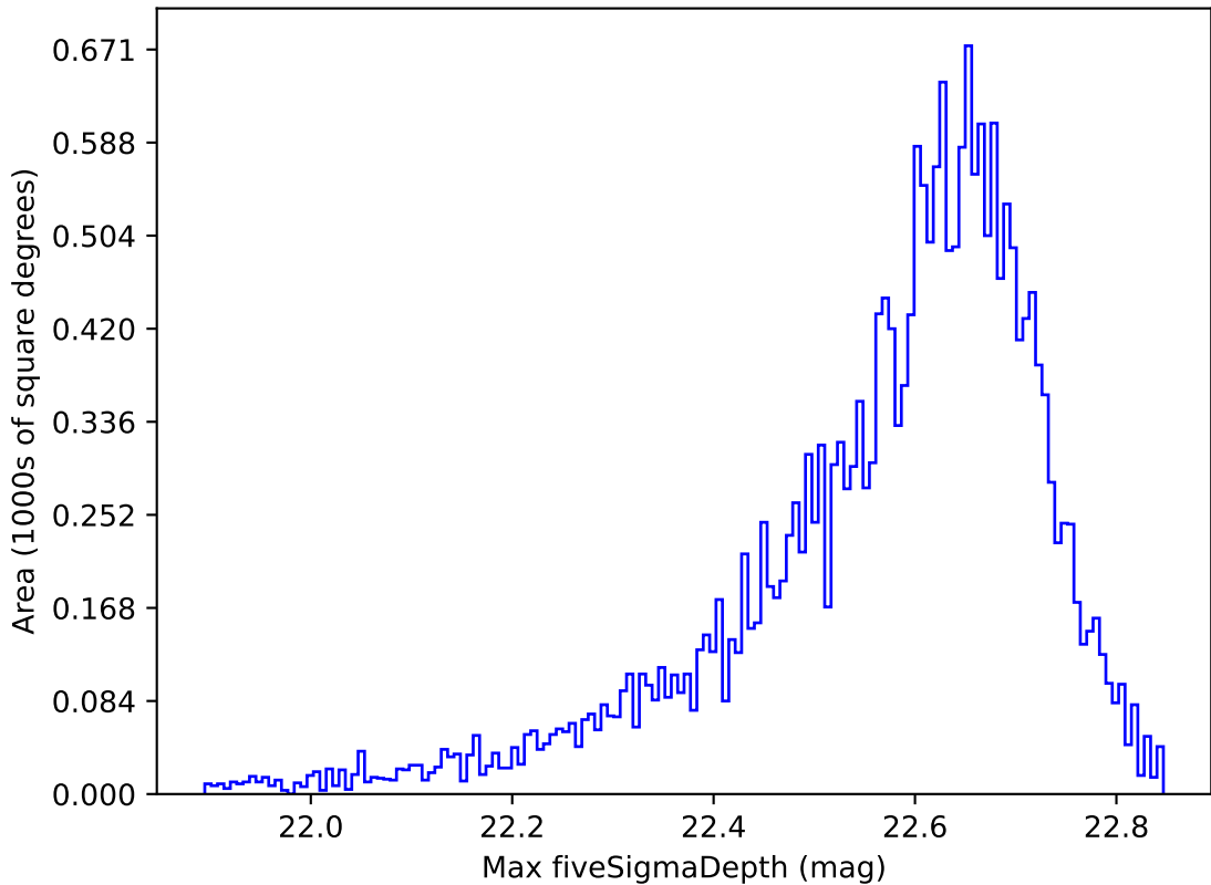
ddf_loaded_half_fl1_v3.4_10yrs All sky y band: Max fiveSigmaDepth
