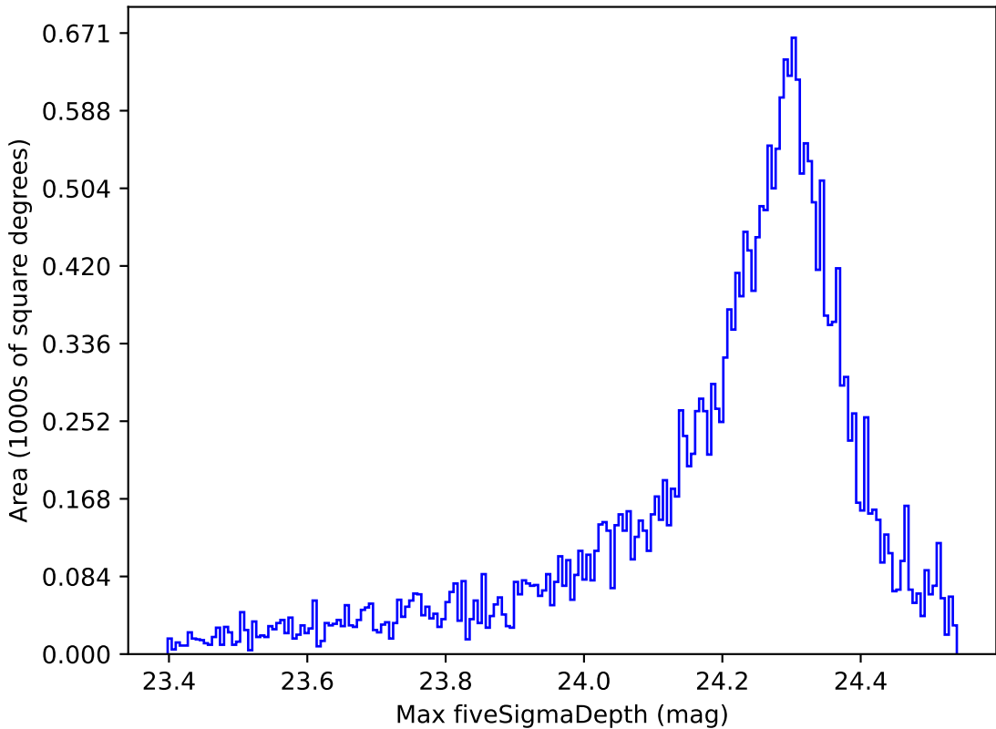
ddf_loaded_half_fl1_v3.4_10yrs All sky i band: Max fiveSigmaDepth
