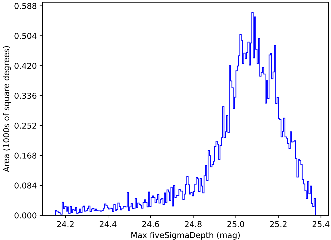
ddf_loaded_half_fl1_v3.4_10yrs All sky g band: Max fiveSigmaDepth
