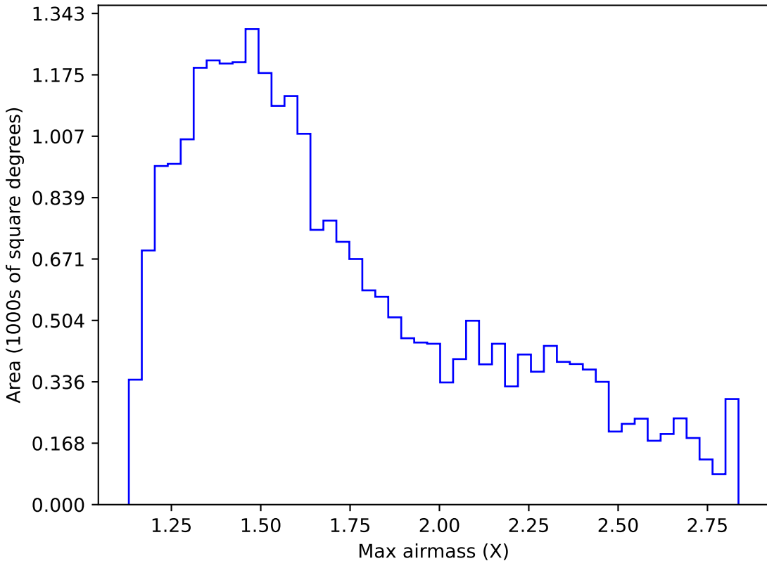
ddf_loaded_half_fl1_v3.4_10yrs Yr 1 z band: Max airmass
