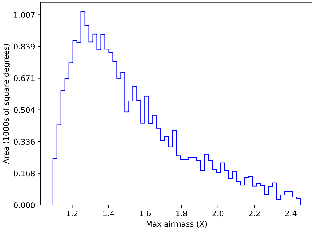
ddf_loaded_half_fl1_v3.4_10yrs Yr 1 u band: Max airmass
