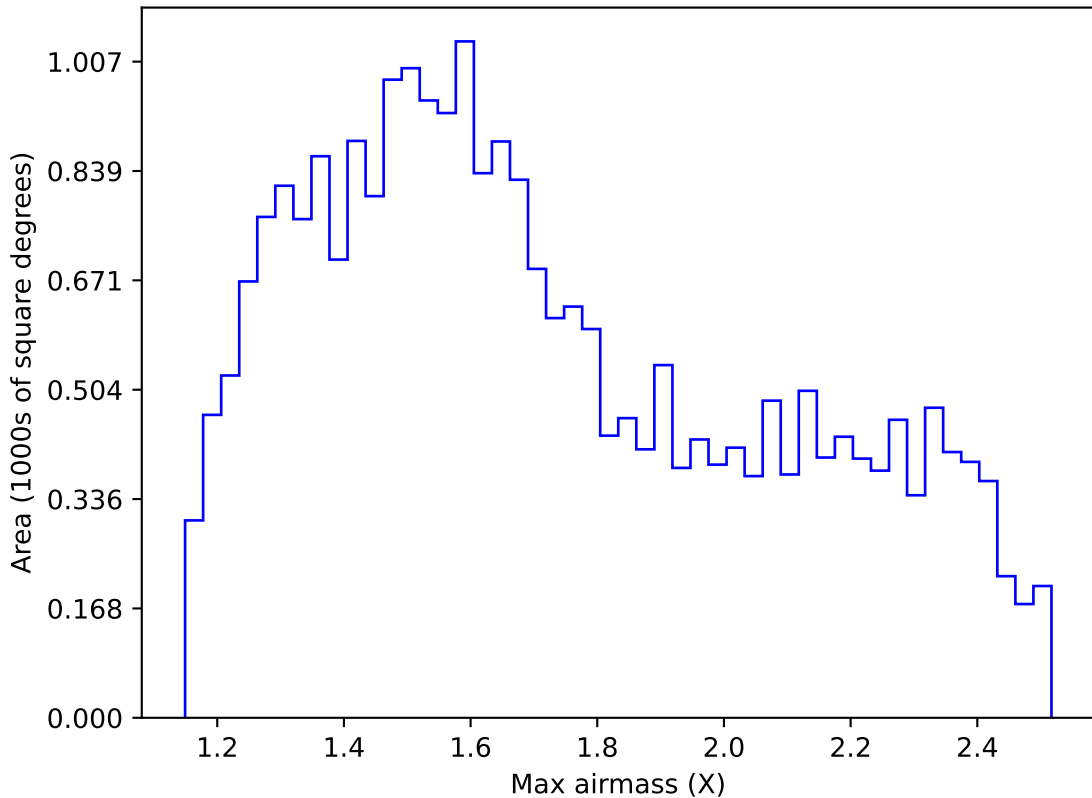
ddf_loaded_half_fl1_v3.4_10yrs Yr 1 r band: Max airmass
