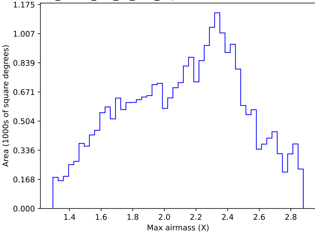
ddf_loaded_half_fl1_v3.4_10yrs Yr 1 all bands: Max airmass
