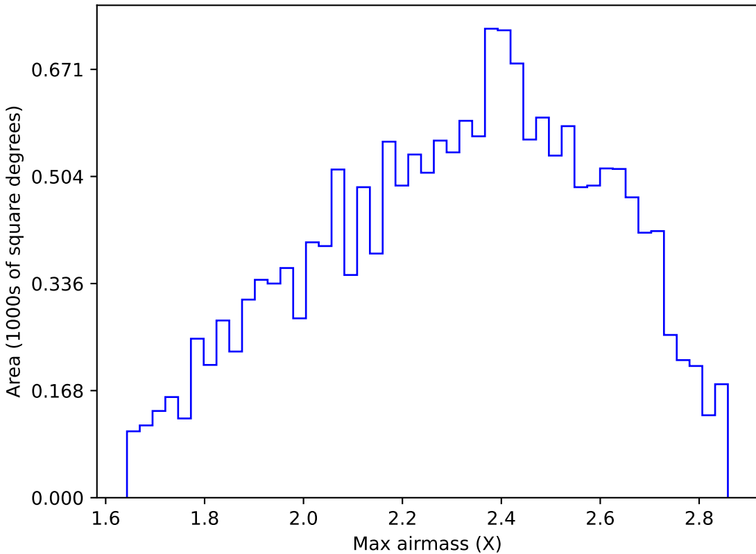
ddf_loaded_half_fl1_v3.4_10yrs WFD y band: Max airmass
