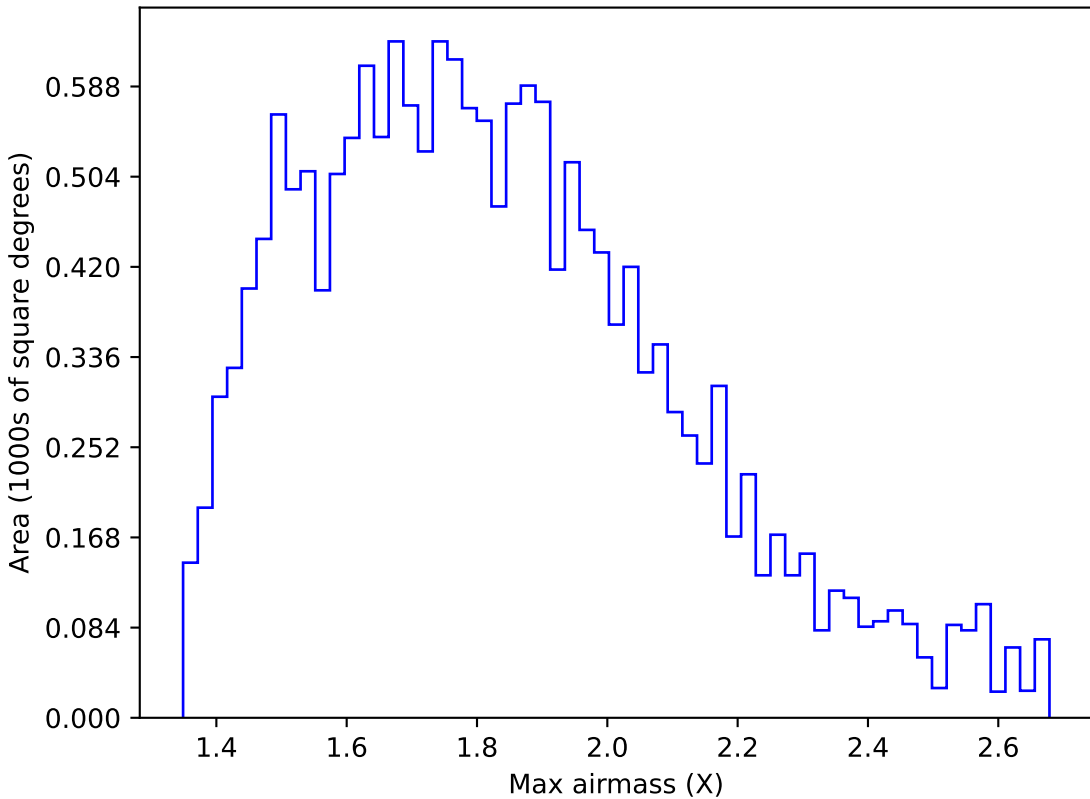
ddf_loaded_half_fl1_v3.4_10yrs WFD u band: Max airmass
