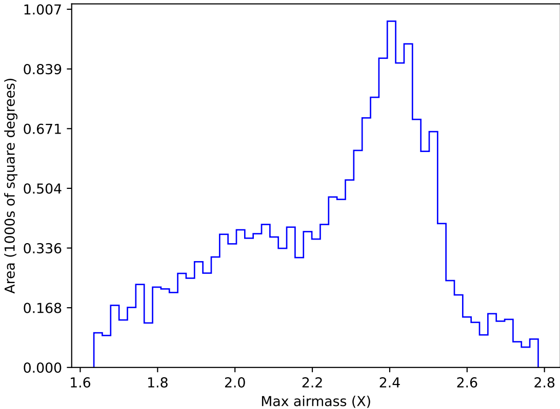
ddf_loaded_half_fl1_v3.4_10yrs WFD r band: Max airmass
