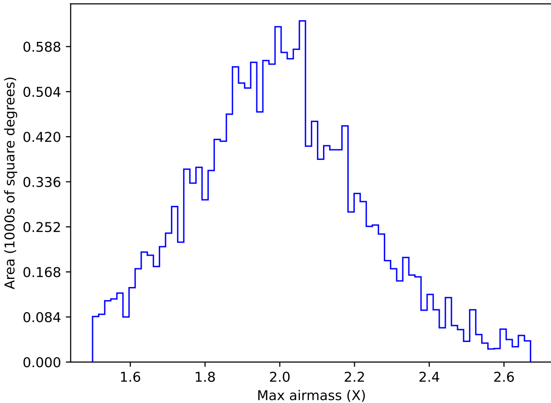
ddf_loaded_half_fl1_v3.4_10yrs WFD g band: Max airmass
