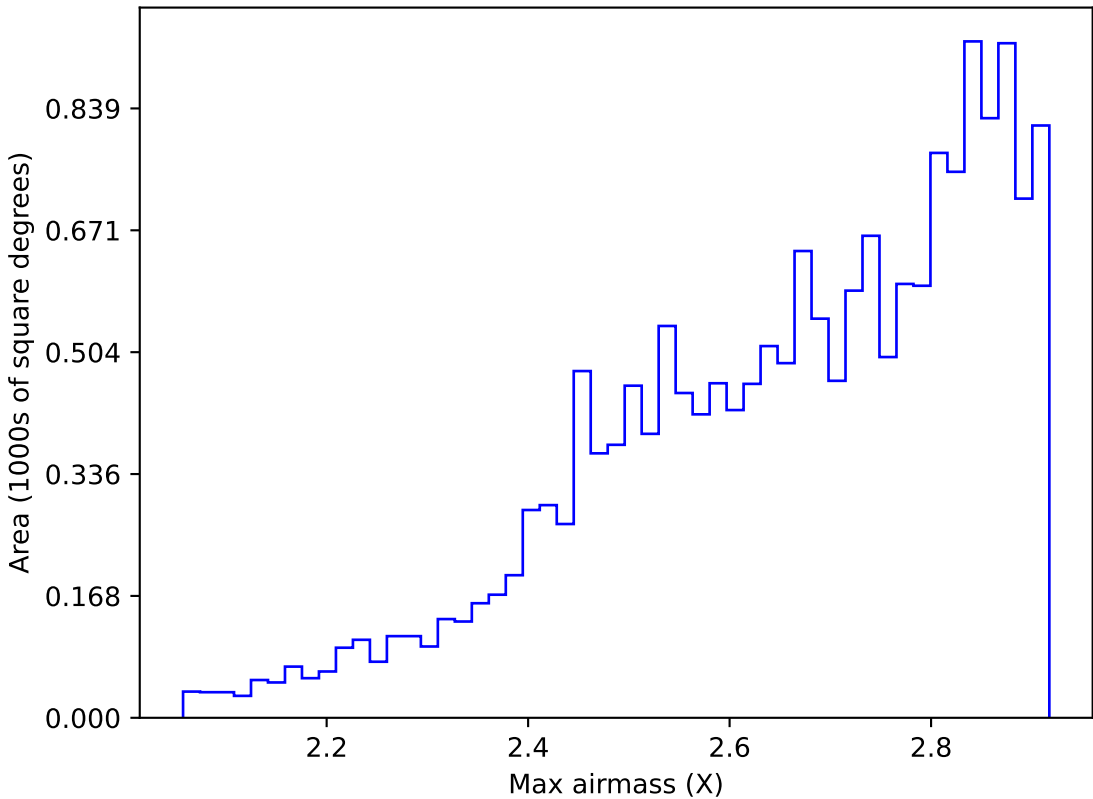
ddf_loaded_half_fl1_v3.4_10yrs WFD all bands: Max airmass
