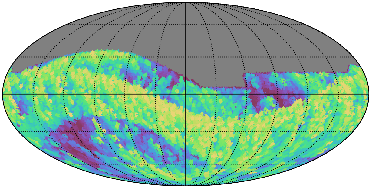
ddf_loaded_half_fi1_v3.4_10yrs All sky z band: Max airmass
