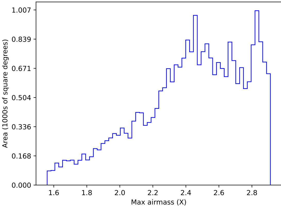
ddf_loaded_half_fl1_v3.4_10yrs All sky z band: Max airmass
