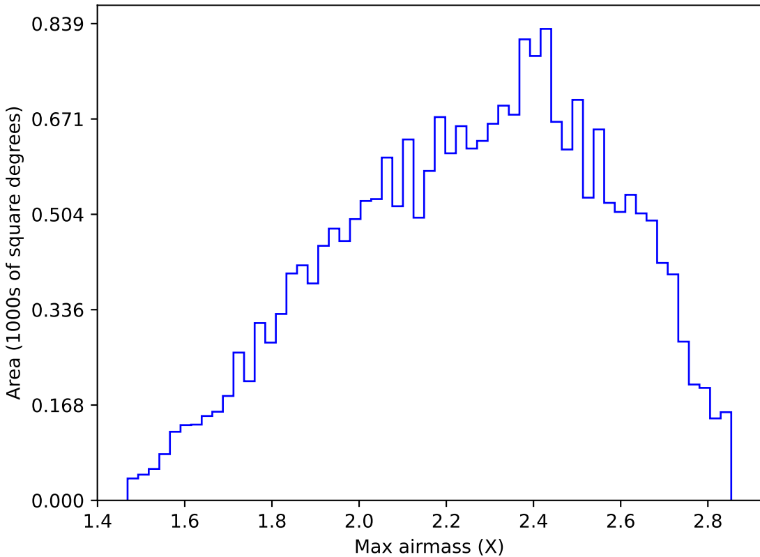
ddf_loaded_half_fl1_v3.4_10yrs All sky y band: Max airmass
