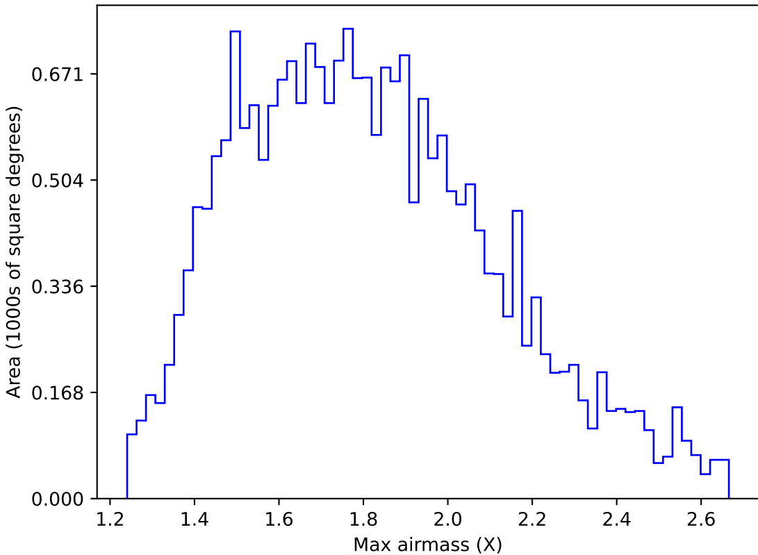
ddf_loaded_half_fl1_v3.4_10yrs All sky u band: Max airmass
