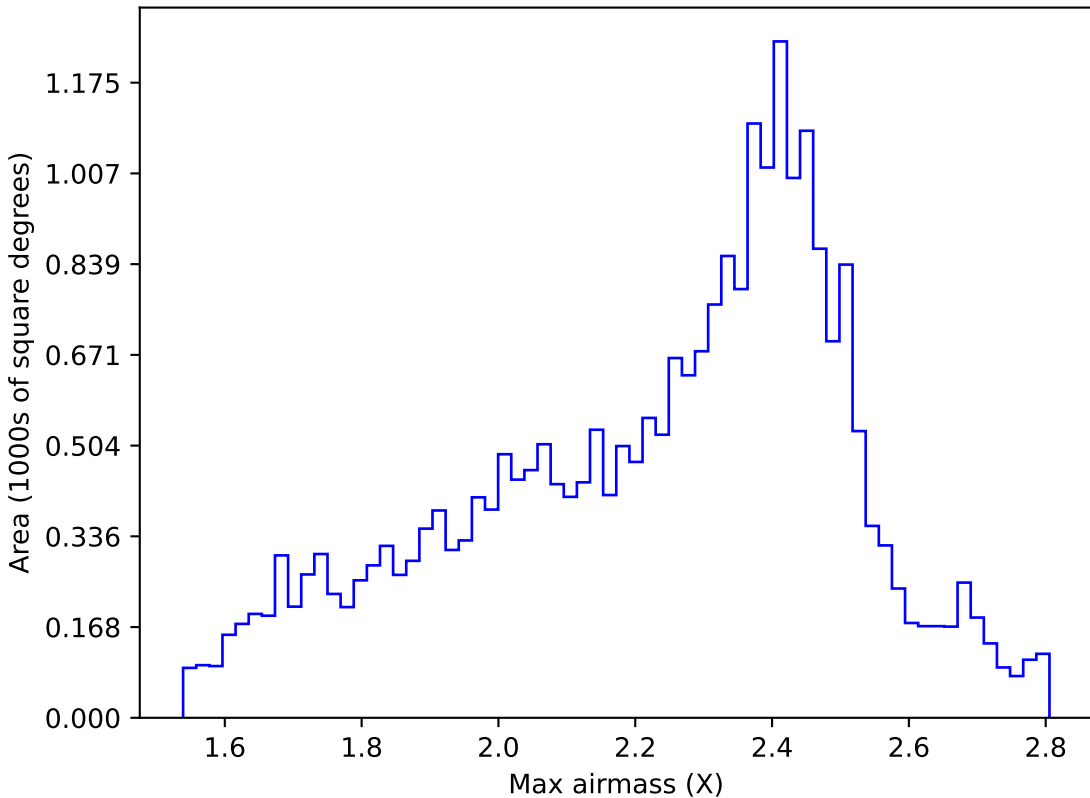
ddf_loaded_half_fl1_v3.4_10yrs All sky r band: Max airmass
