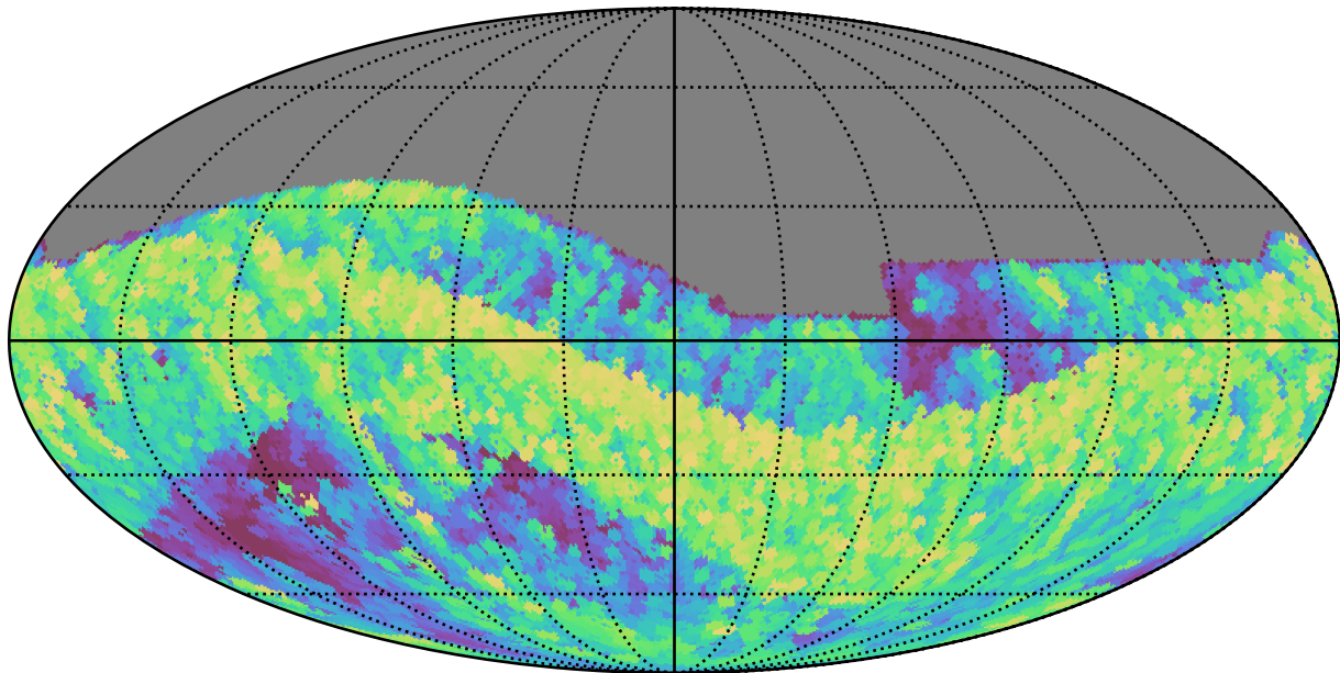
ddf_loaded_half_fl1_v3.4_10yrs All sky i band: Max airmass
