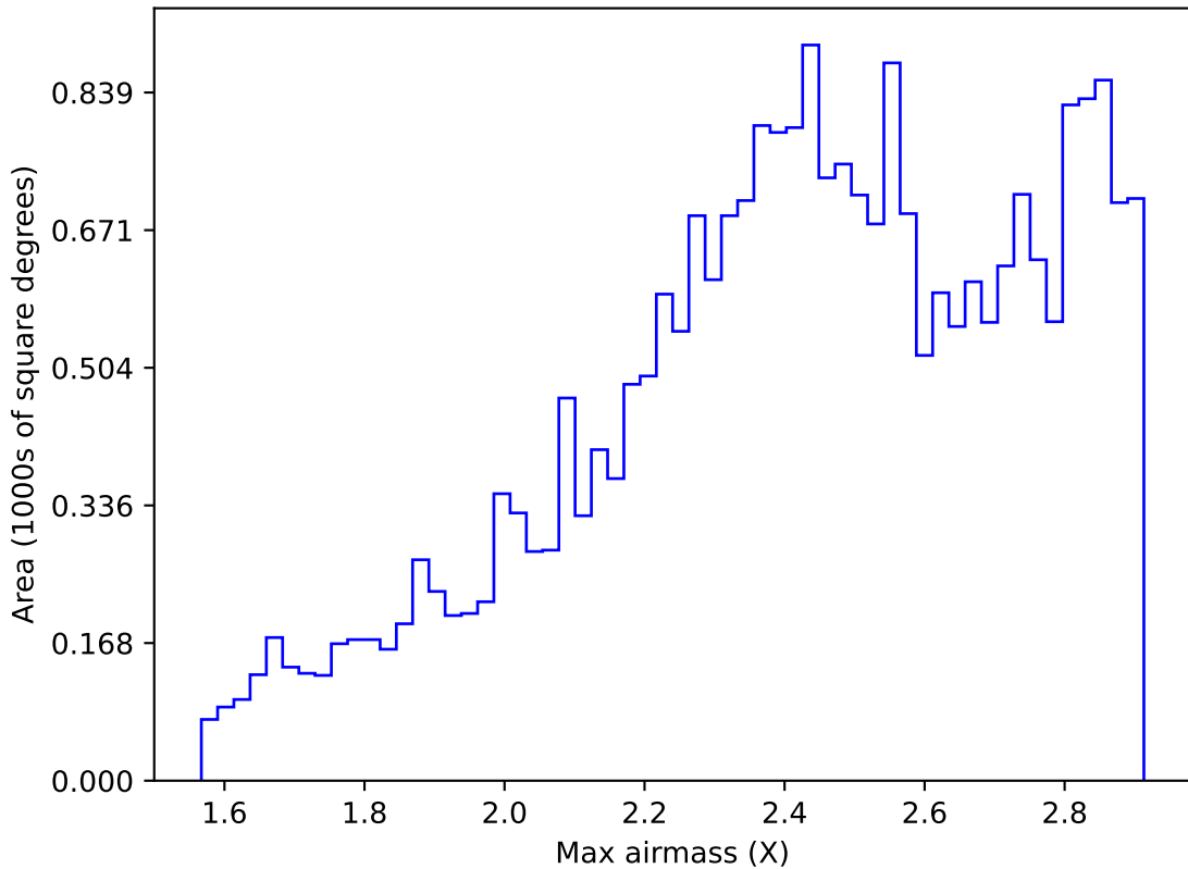
ddf_loaded_half_fl1_v3.4_10yrs All sky i band: Max airmass
