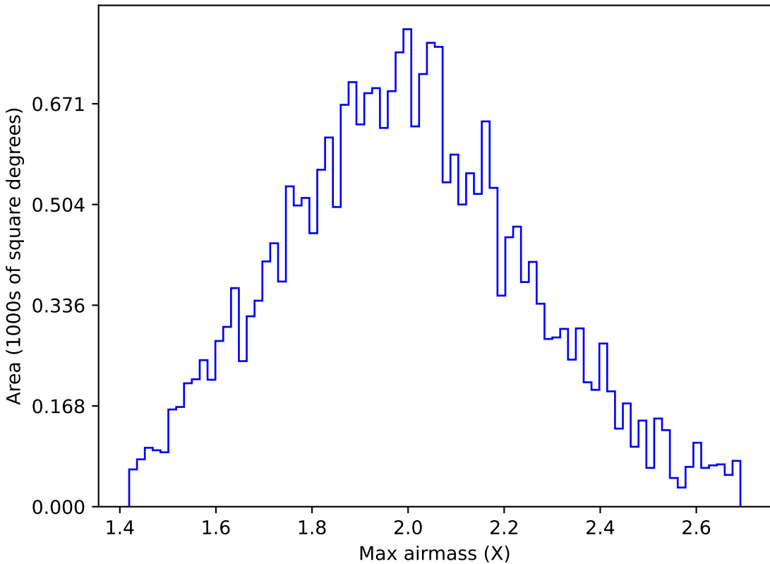
ddf_loaded_half_fl1_v3.4_10yrs All sky g band: Max airmass
